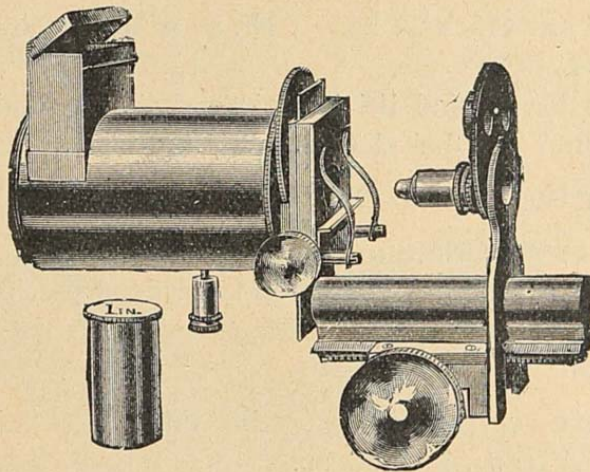
Grosses Microscop Modell II.
